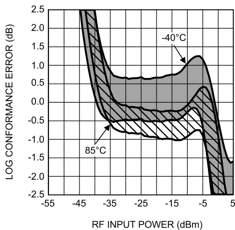
Log Conformance Error (Mean \pm 3 sigma) vs. RF Input Power at 3000 MHz
