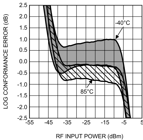
Log Conformance Error (Mean \pm 3 sigma) vs. RF Input Power at 1855 MHz
